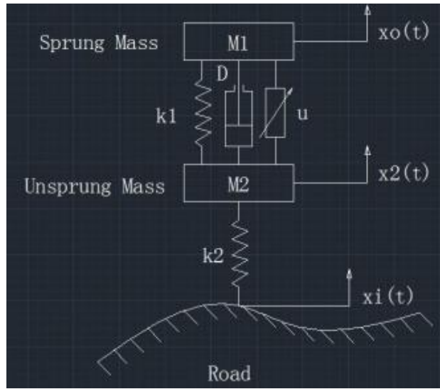
Figure 4: 1/4 active suspension system model with actuation force ( u ) between springs [24]
