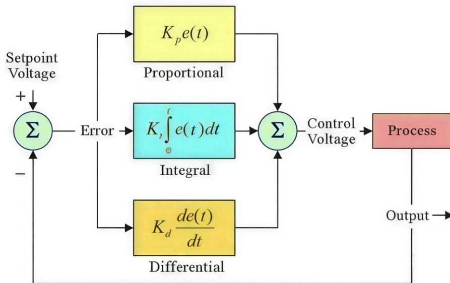
Figure 1: Block diagram from PID controller [6]
