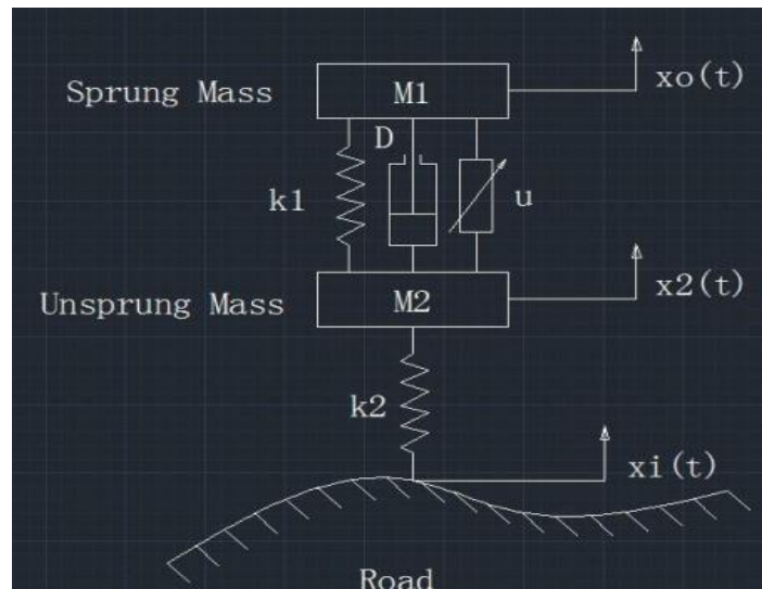
Figure 6: Modelling active suspension with actuating force ( u ) between sprung and unsprung mass [24]
