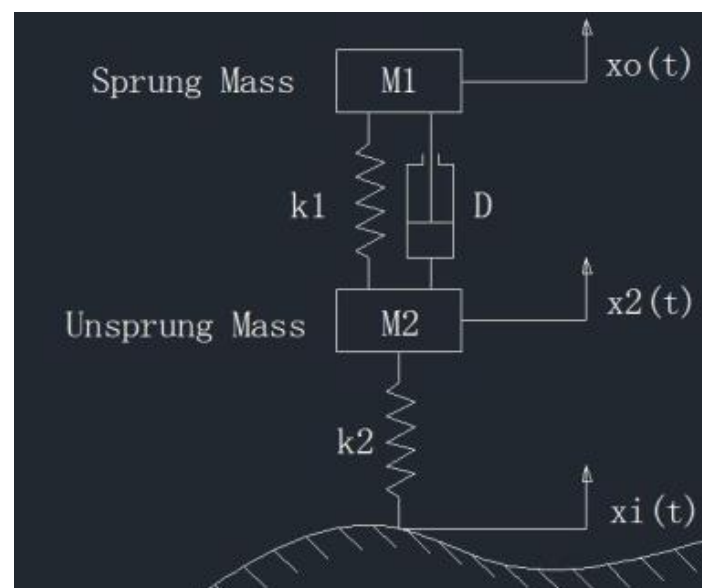
Figure 7: Math model of passive suspension system [24]
