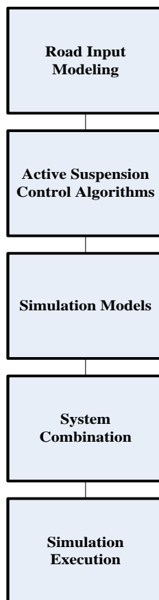
Figure 3: Flow chart of methodology for active suspension simulations in MATLAB
