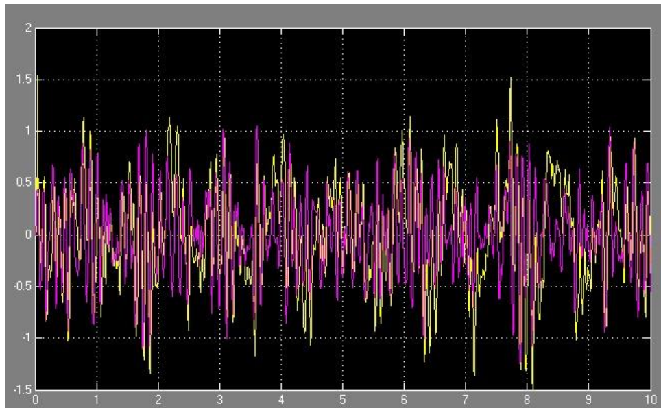
Figure 11: New algorithm compares active suspension system acceleration time response to passive suspension system with white noise signal input [24]
