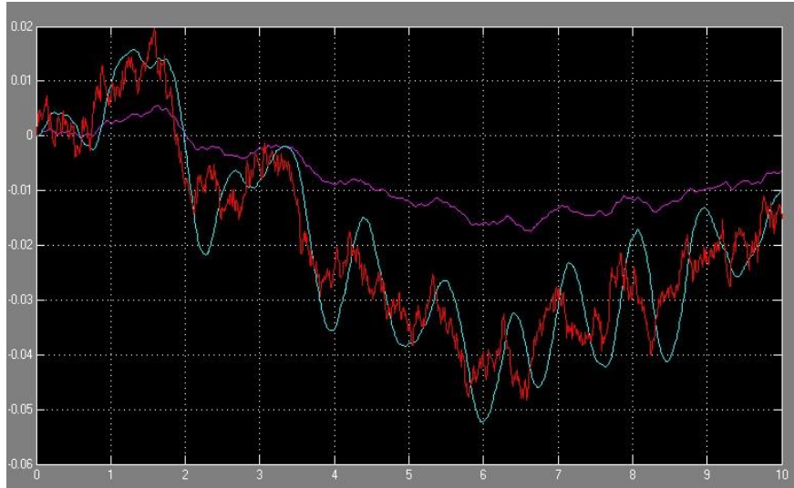
Figure 12: New algorithm PID control active suspension output displacement time response with white noise signal input compared to passive suspension [24]
